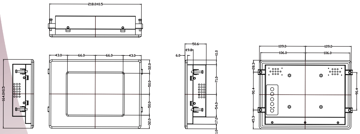
CUT OUT DIMENSION(191x142mm) UNIT:mm
